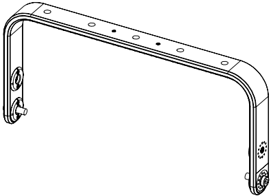
VNU-HBRK365 bracket for ePS6 VNU-HBRK425 bracket for ePS8 VNU-HBRK535 bracket for ePS10 Horizontal mounting bracket
